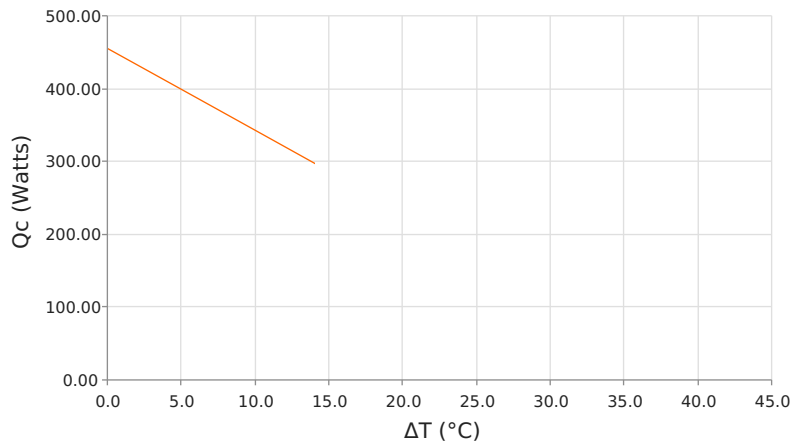
Heat Pumped at Cold Side (Qc) Voperating = 48.2 Volts | Ioperating = 8.8 Amps
