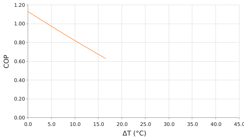
Coefficient of Performance (COP = Qc/Pin) Voperating = 48.2 Volts | Ioperating = 8.8 Amps
