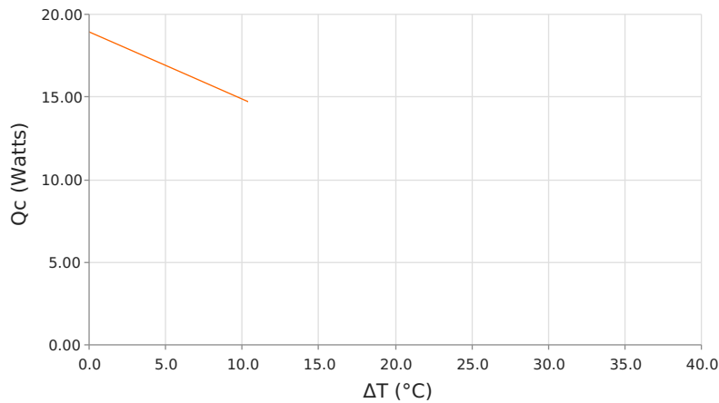
Heat Pumped at Cold Side (Qc) Voperating = 0 Volts | Ioperating = 0 Amps
