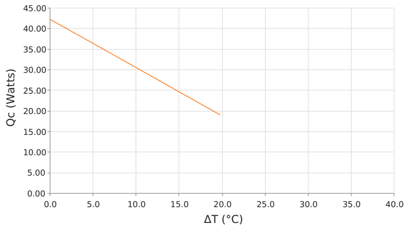
Heat Pumped at Cold Side (Qc) Voperating = 24.1 Volts | Ioperating = 2.4 Amps
