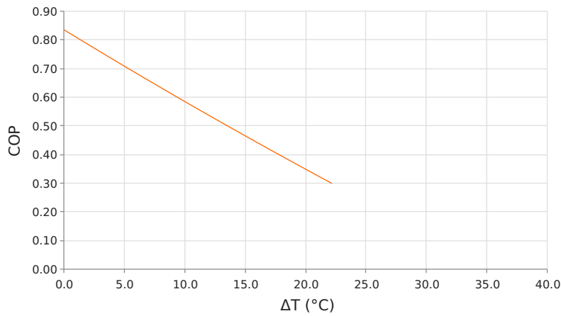
Coefficient of Performance (COP = Qc/Pin) Voperating = 24.1 Volts | Ioperating = 2.4 Amps
