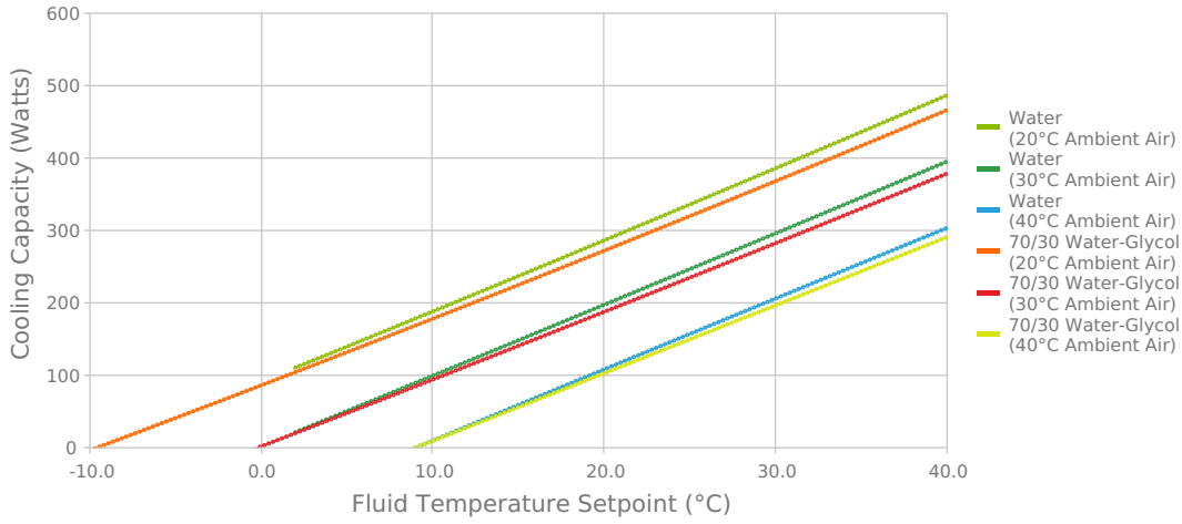
MRC300-DH2-DV \Delta T (Inlet-Outlet) Fluid Temperature
