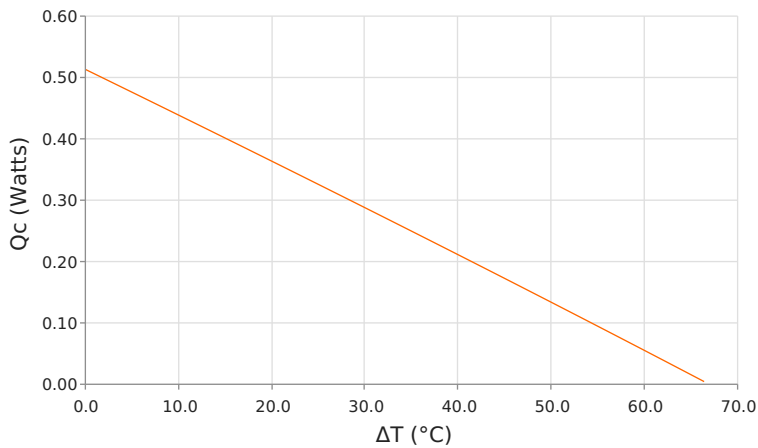
Heat Pumped at Cold Side (Qc) Thot = 27 °C | Current = 0.7 Amps
