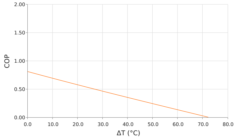
Coefficient of Performance (COP = Qc/Pin) Thot = 27 °C | Current = 9.6 Amps
