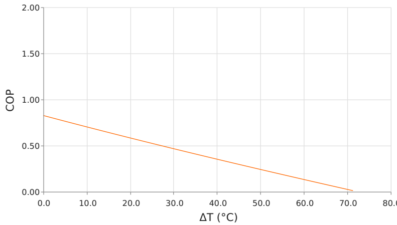
Coefficient of Performance (COP = Qc/Pin) Thot = 35 °C | Ioperating = 5.1 Amps
