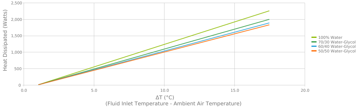
WL1500 Fluid Inlet/Outlet Temperature Difference (ΔT) @ Nominal Flow 6 L/min
