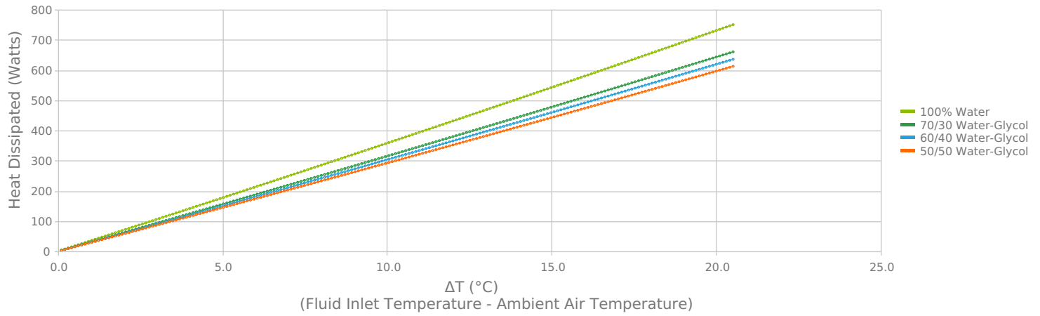
WL500 Fluid Inlet/Outlet Temperature Difference ( \Delta T ) @ Nominal Flow 2.3 L/min
